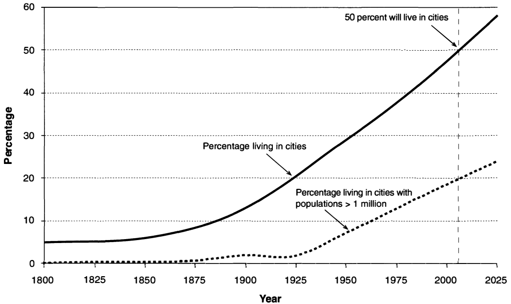
Figure 3. Trends in World Urbanization, 1800 to 2000
